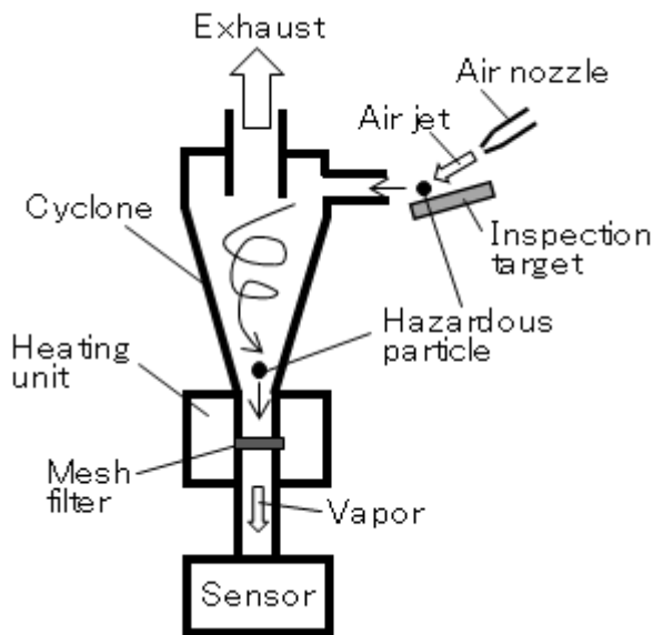
Diagram of hazardous material inspection system
